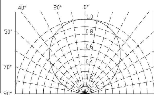
Curves of beam angle and relative brightness
